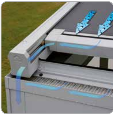
Integrated water channels
